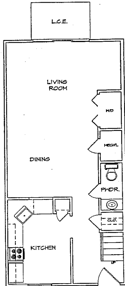
3 BDRM DELUXE END UNIT FIRST FLR. PLAN (REV.)
