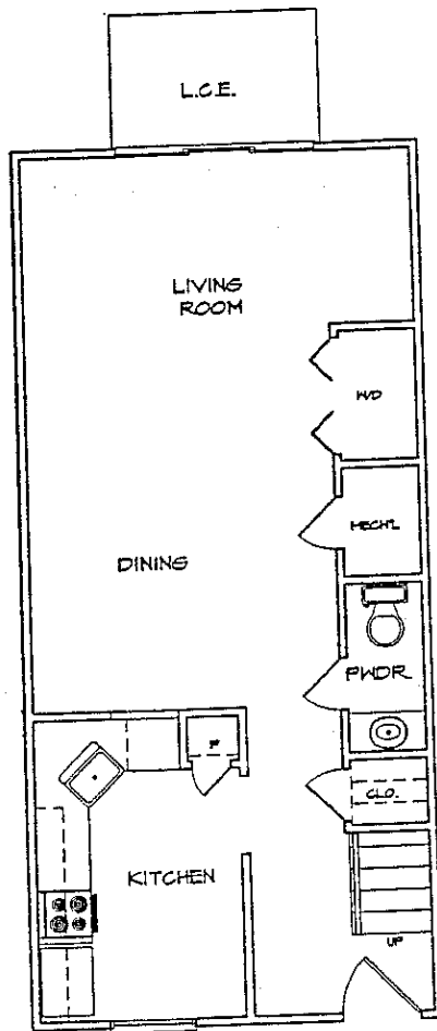
TWO BEDROOM UNIT FIRST FLR PLAN (REV.)
