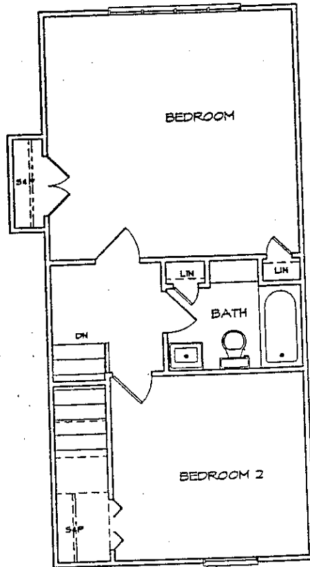
7 A-38 TWO BEDROOM UNIT SECOND FLOOR PLAN SCALE: 1/8" = 1'-0"
