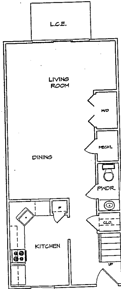
3 BEDROOM UNIT FIRST FLR PLAN (REV.)
